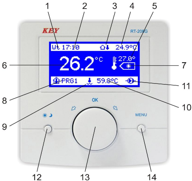
Picture 1. Front cover of the RT-208G controller.
