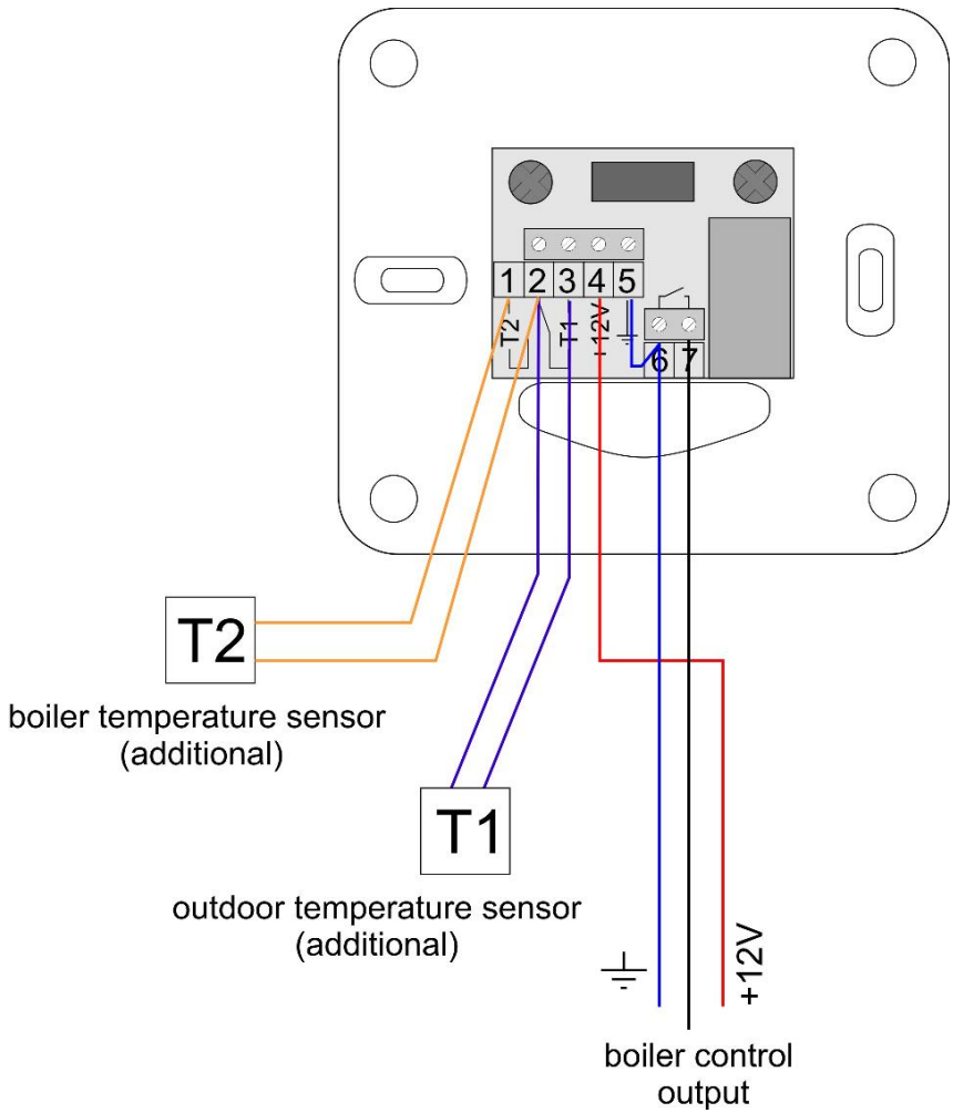
Connection diagram of the RT-208G regulator with a three-core cable to the boiler regulator (boiler boiler control).
