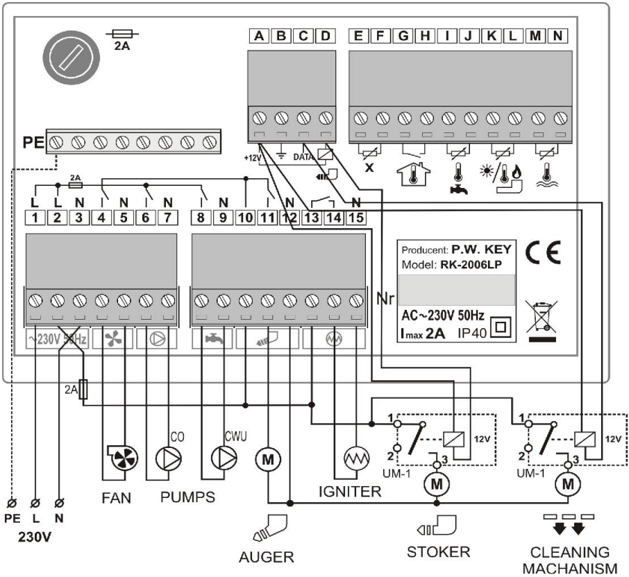
Figure 2. RK-2006LPP Controller connection diagram.
